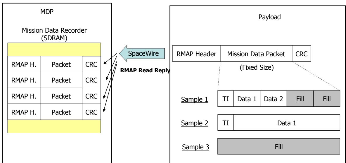
Fig. 5.7 Mission Data Packet (example)
