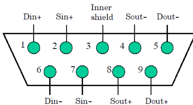
Fig. 4.1 Standard pin assignment of the SpW connector for Payloads (u-Sub 9pin: Socket type) [Ref. ECSS-E-50-12A]
