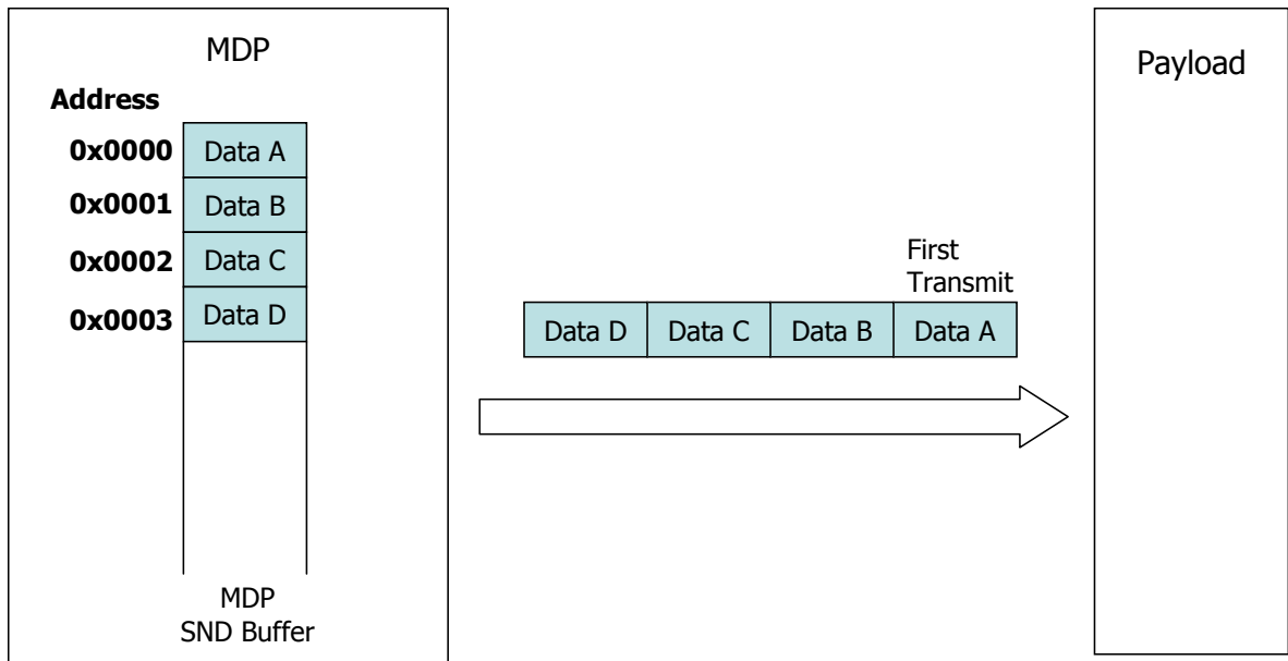
Fig. 4.3 Data Send Scheme fo the Payload
