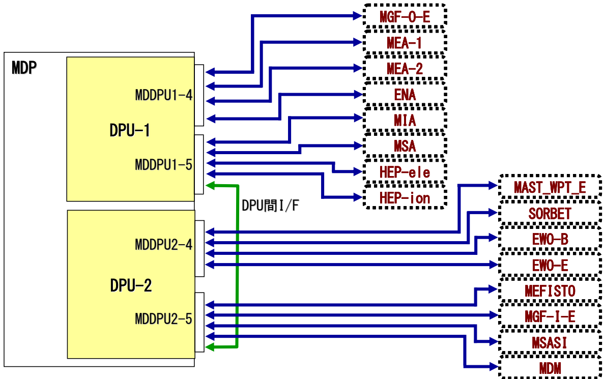
Fig. 3.1 MDP-Payload SpaceWire Interface design
