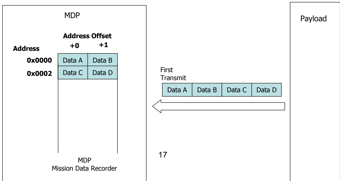
Fig. 4.4 Data Receive Scheme from the Payload
